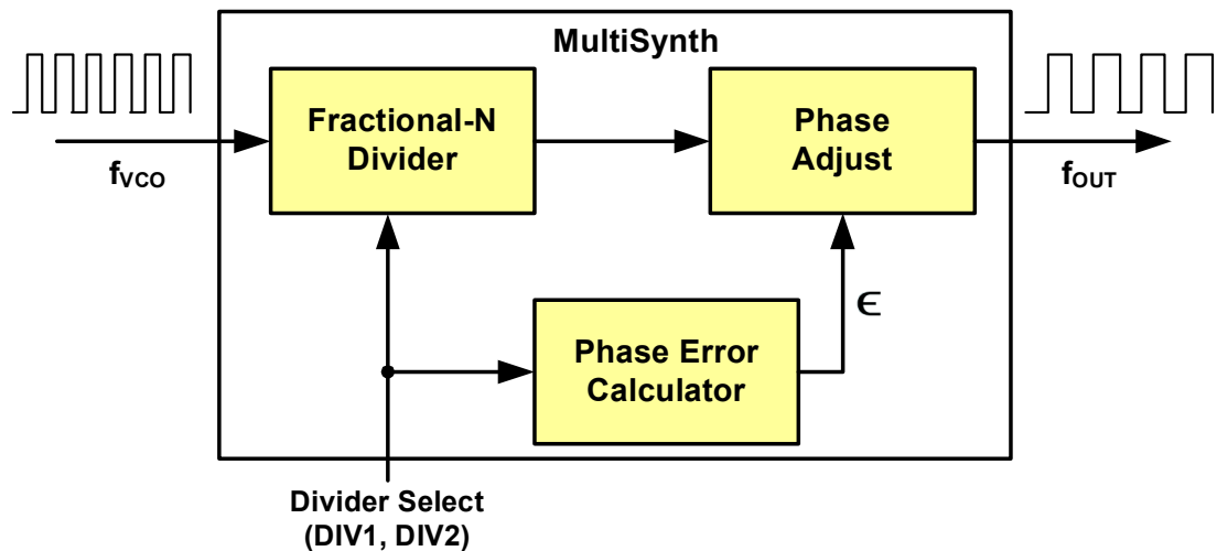
Figure 2. Skyworks Solutions’ MultiSynth Technology
