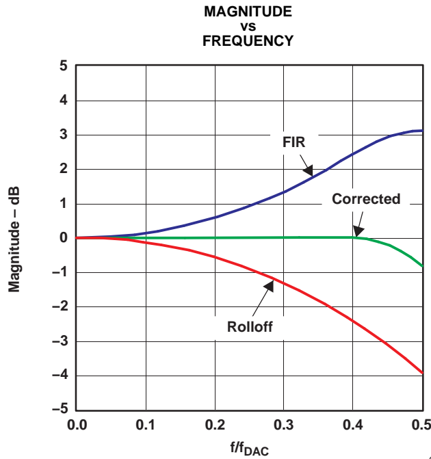
Figure 43. Magnitude Spectrum for Inverse sinc Filtering
