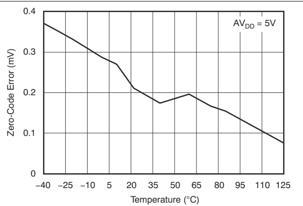
Figure 7-9. Zero-Code Error vs Temperature
