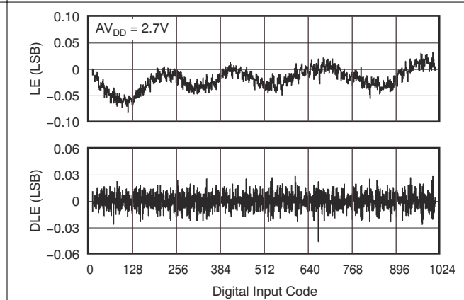
Figure 7-45. DAC6311 10-Bit Linearity Error and Differential Linearity Error vs Code ( -40^\circ\text{C} )
