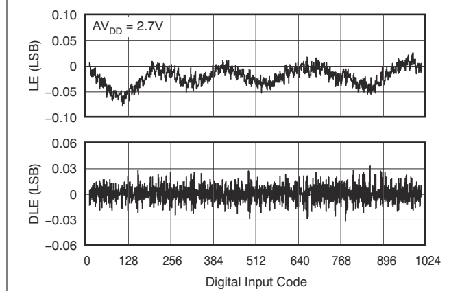
Figure 7-47. DAC6311 10-Bit Linearity Error and Differential Linearity Error vs Code ( 25^\circ\text{C} )
