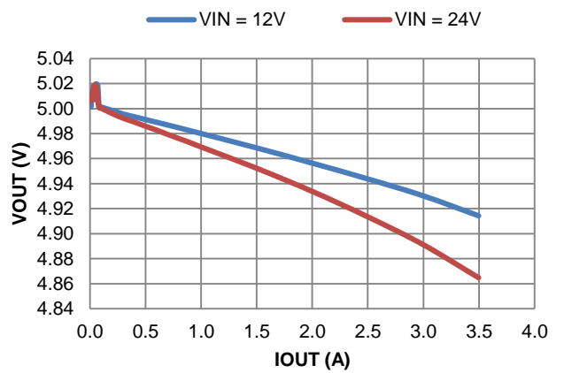
Figure 28. Load Regulation
