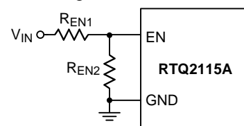
Figure 21. Resistive Divider for Under-Voltage Lockout Threshold Setting
