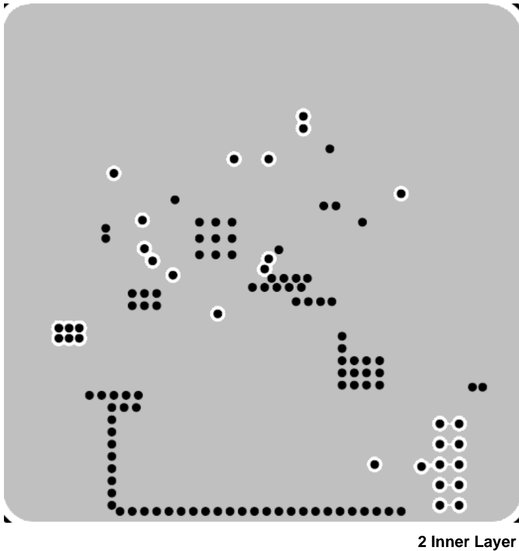
Figure 26. Layout Guide (2 Inner Layer)
