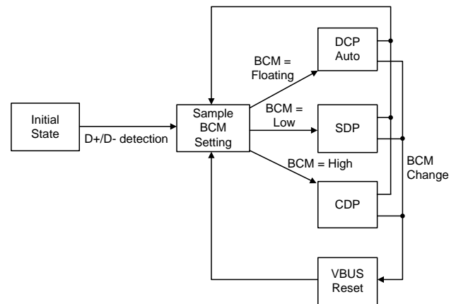
Figure 23. Detection Flow
