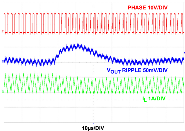
FIGURE 38. CCM TO DCM TRANSITION
