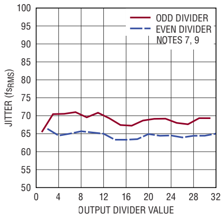
Additive Jitter vs Divider Setting, ADC SNR Method
