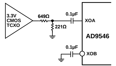
Figure 31. System Clock Input (XOA, XOB) Using the Direct Path with a TCXO or Oven Controlled Crystal Oscillator (OCXO) Having a 3.3 V CMOS Output
