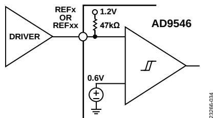
Figure 34. Single-Ended Internal Pull-Up Resistor Mode
