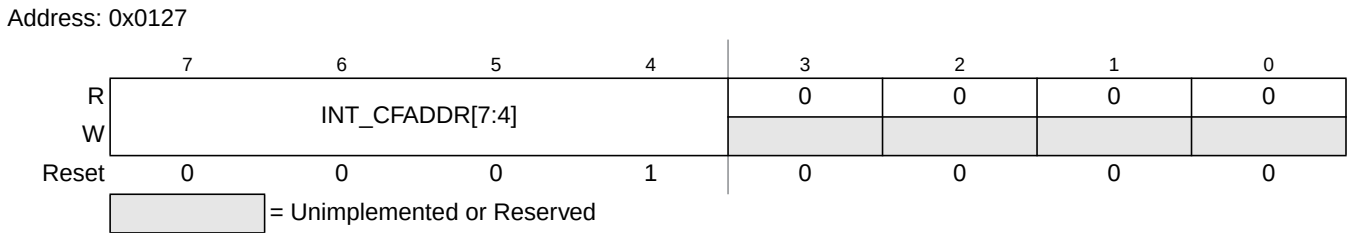
Figure 24-5. Interrupt Configuration Address Register (INT_CFADDR)
