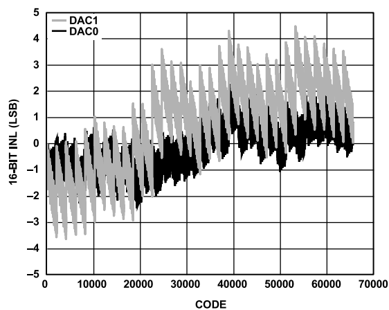
Figure 13. INL, I_{OUTFS} = 26 mA, 16-Bit Resolution
