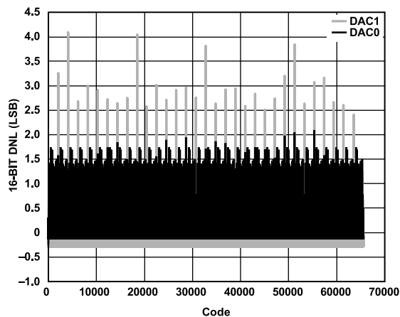
Figure 14. DNL, I_{OUTFS} = 20 mA, 16-Bit Resolution
