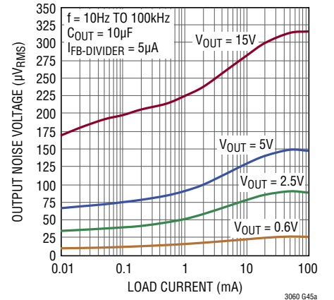
RMS Output Noise vs Load Current C_{REF/BYP} = 10\text{nF}, C_{FF} = 0
