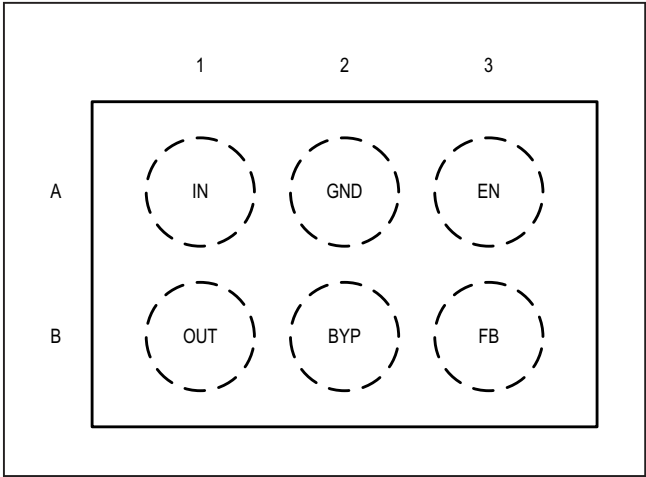
MAX38902C TOP VIEW (BUMP-SIDE DOWN)
