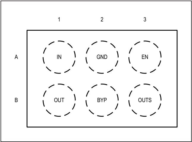
MAX38902D TOP VIEW (BUMP-SIDE DOWN)
