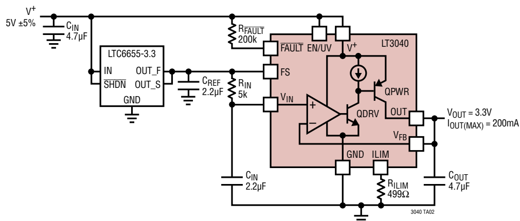
200mA 3.3V Precision Reference
