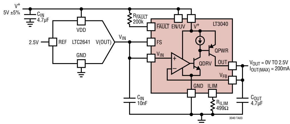
200mA 0V to 2.5V Precision DAC
