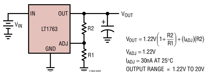
Figure 2. Adjustable Operation
