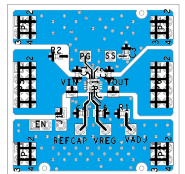
Figure 47. Typical Board Layout, Top Side
