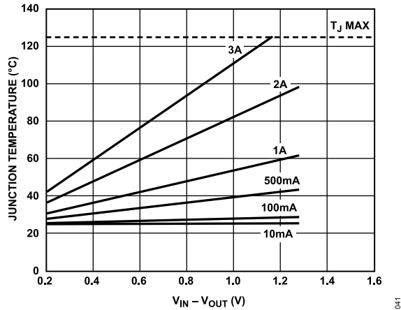
Figure 43. 1000 mm 2 of PCB Copper, T_B = 25^\circ\text{C}
