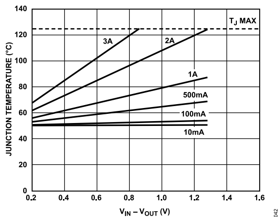
Figure 44. 1000 mm 2 of PCB Copper, T_B = 50^\circ\text{C} , LFCSP
