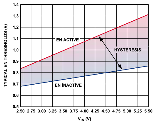
Figure 32. Typical EN Pin Thresholds vs. Input Voltage
