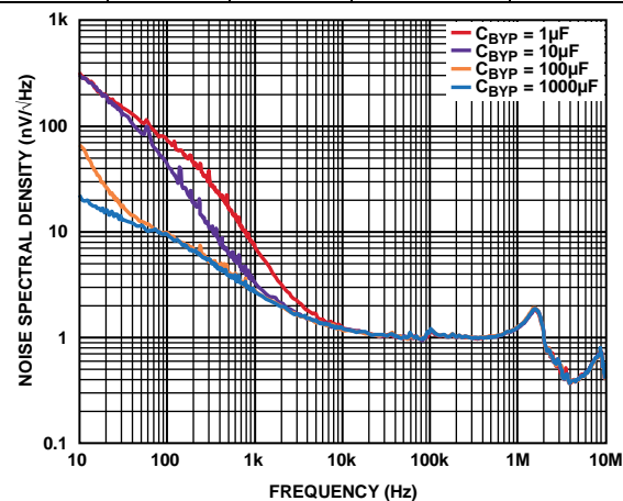
Figure 2. Noise Spectral Density at Different Values of C_{BYP} , V_{OUT} = 3.3 \text{ V}
