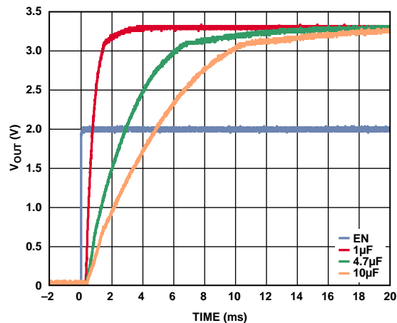
Figure 53. Typical Start-Up Behavior with C_{BYP} = 1 \mu F
