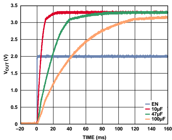
Figure 54. Typical Start-Up Behavior with C_{BYP} = 1 \mu F to 100 \mu F
