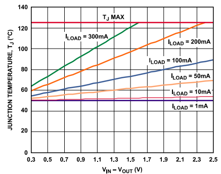
Figure 34. 100 mm 2 of PCB Copper, T_A = 50^\circ\text{C}
