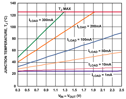
Figure 32. 0 mm 2 of PCB Copper, T_A = 25^\circ\text{C}
