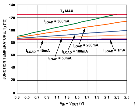
Figure 36. T A = 85°C
