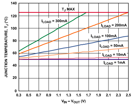
Figure 33. 500 mm 2 of PCB Copper, T_A = 50^\circ\text{C}
