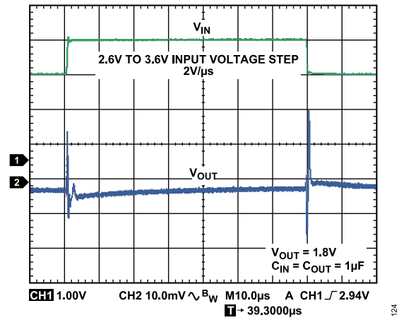
Figure 22. Line Transient Response, Load Current = 300 mA
