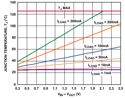
Figure 31. 100 mm 2 of PCB Copper, T_A = 25^\circ\text{C}
