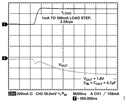
Figure 25. Output Transient Response, C_{OUT} = 4.7 \mu\text{F}
