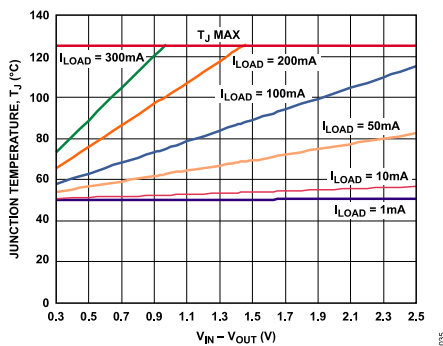
Figure 35. 0 mm 2 of PCB Copper, T A = 50°C
