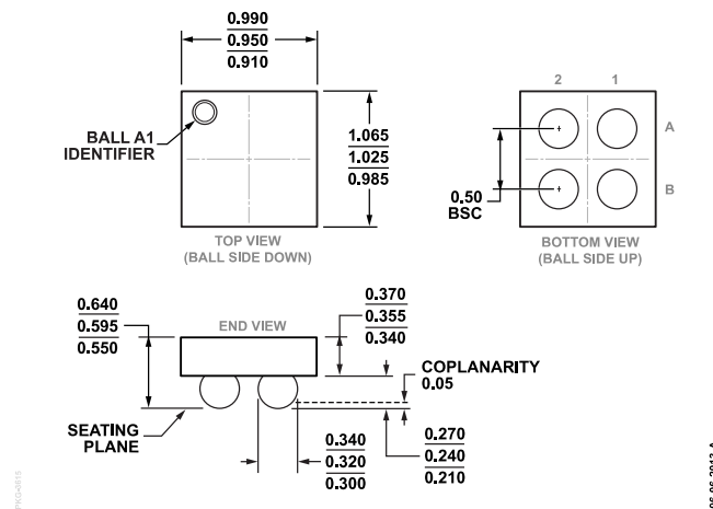
Figure 38. 4-Ball Wafer Level Chip Scale Package [WLCSP] (CB-4-4) Dimensions shown in millimeters
