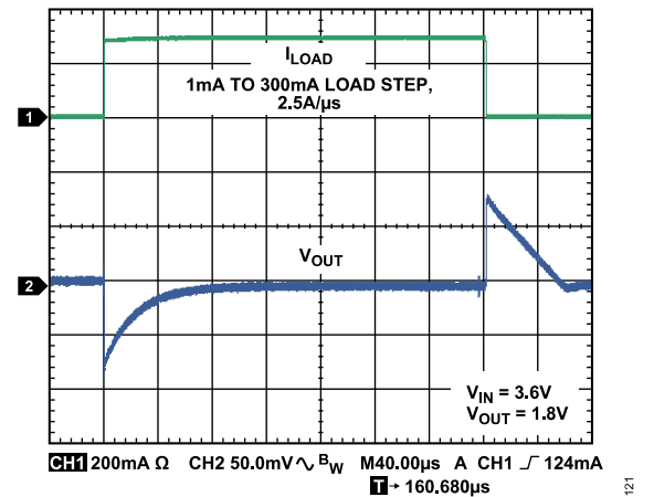
Figure 19. Load Transient Response, C_{IN} and C_{OUT} = 1\ \mu\text{F}
