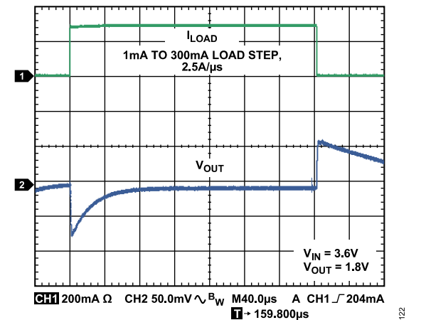
Figure 20. Load Transient Response, C_{IN} and C_{OUT} = 4.7\ \mu\text{F}
