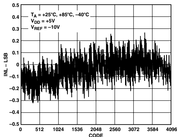
Figure 1. Integral Nonlinearity Error vs. Code
