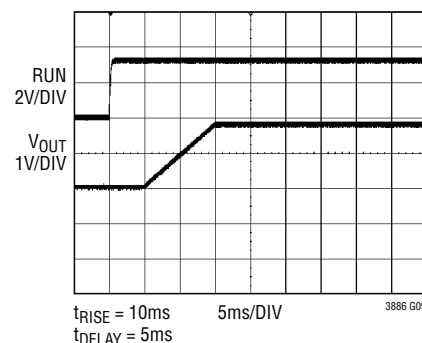
Soft-Start Ramp
