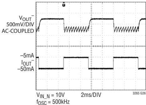
V OUT - Transient (Burst Mode Operation, MODE = H)
