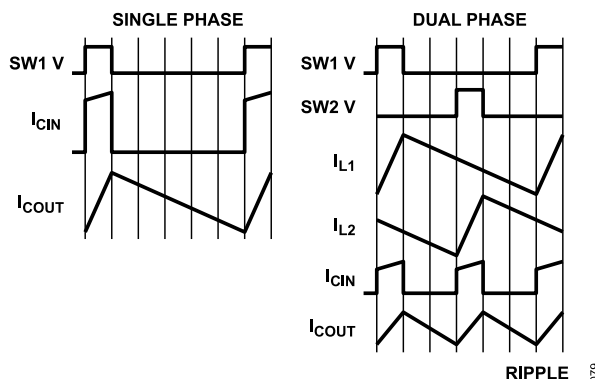
Figure 76. Single and 2-Phase Current Waveforms
