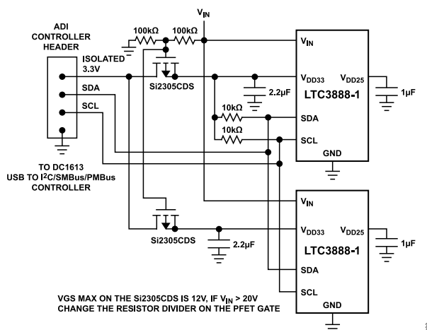
Figure 81. DC1613 Connections
