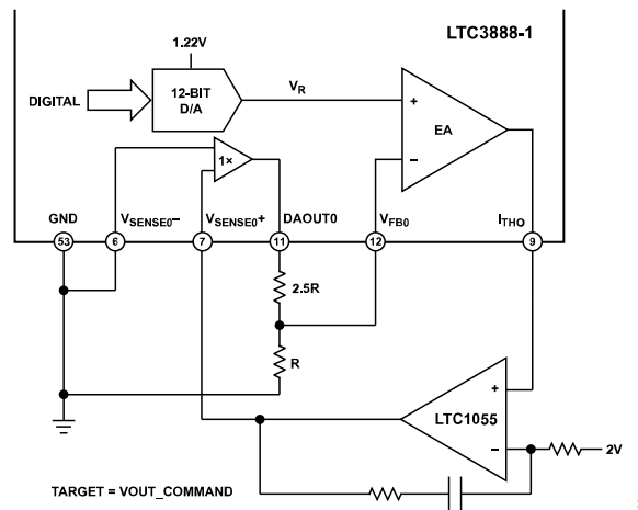
Figure 33. LTC3888-1
