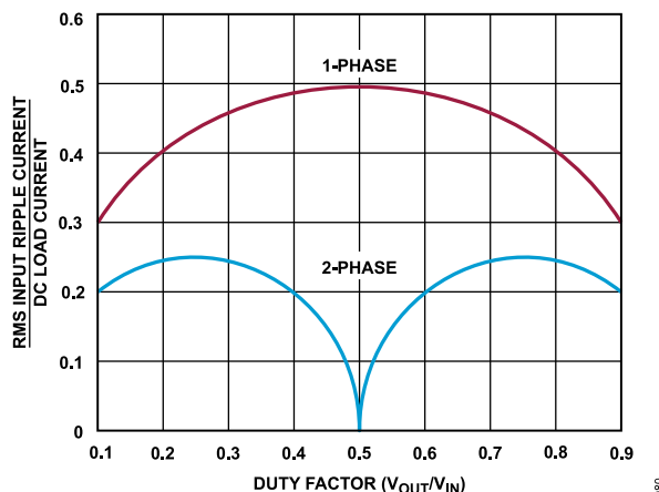
Figure 77. Normalized RMS Input Ripple Current
