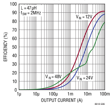
LT8618C: Forced Continuous Mode Efficiency (5V Output)
