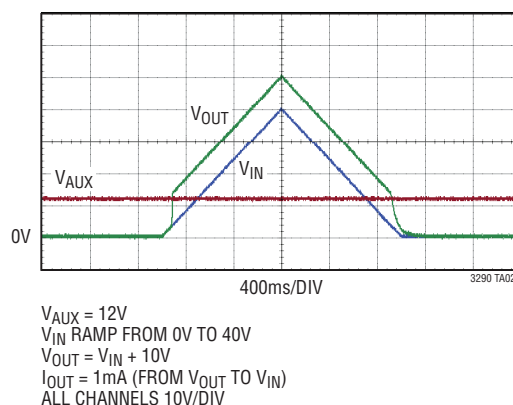
Figure 10. (V IN + 10V) Tracking Power Supply
