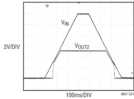
Channel 2 Start-Up and Dropout, R_L = 20\Omega
