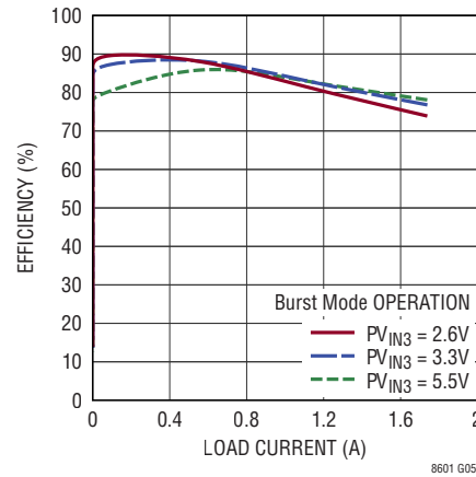
LV Channel Efficiency vs Load V_{OUT3} = 1.2\text{V} , f_{SW} = 2\text{MHz}
