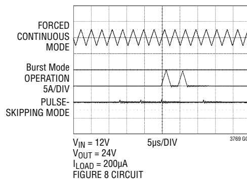
Inductor Currents at Light Load
