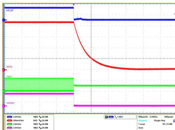
Figure 8-8. Shutdown (immediate off) channel A
