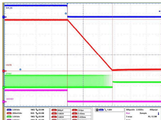
Figure 8-15. Soft-stop channel B (0 ms TOFF_DELAY)
