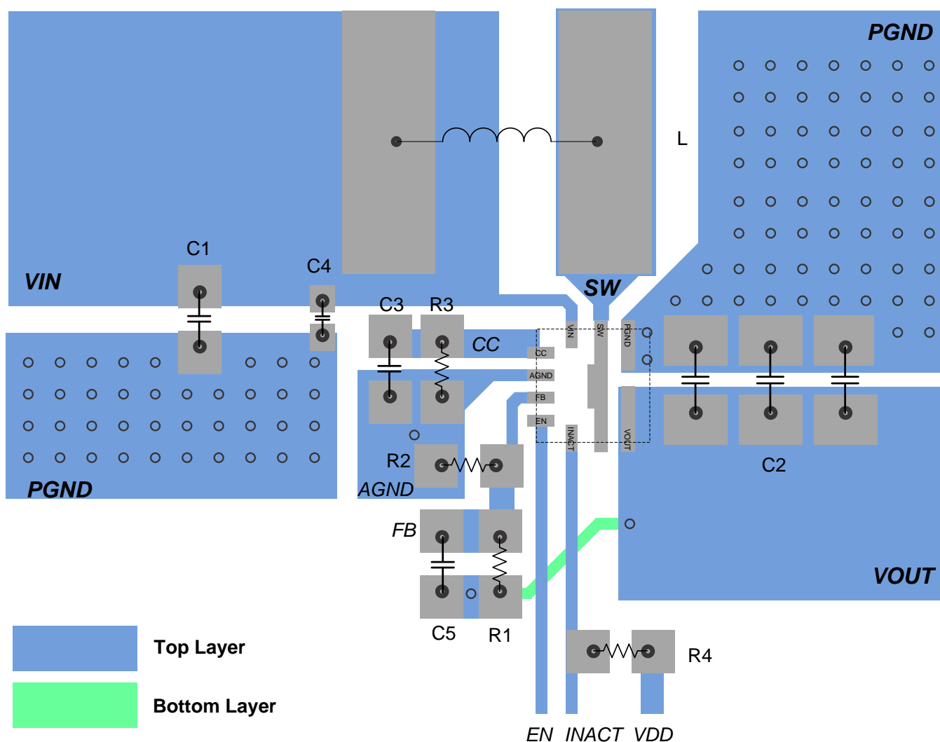
Figure 39. Layout Recommendation
