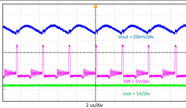
Figure 9-6. Output Voltage Ripple, I_{out} = 0.2\text{ A}
