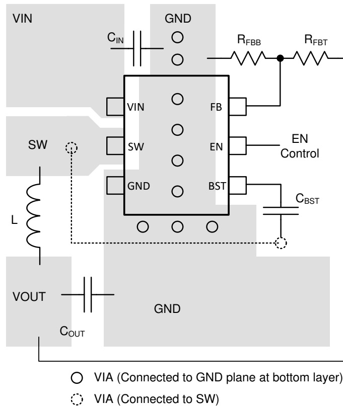
Figure 11-1. TPS562202S Layout
