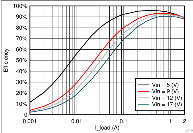
Figure 7-13. V_{OUT} = 3.3 V Efficiency, L = 3.3 μH
