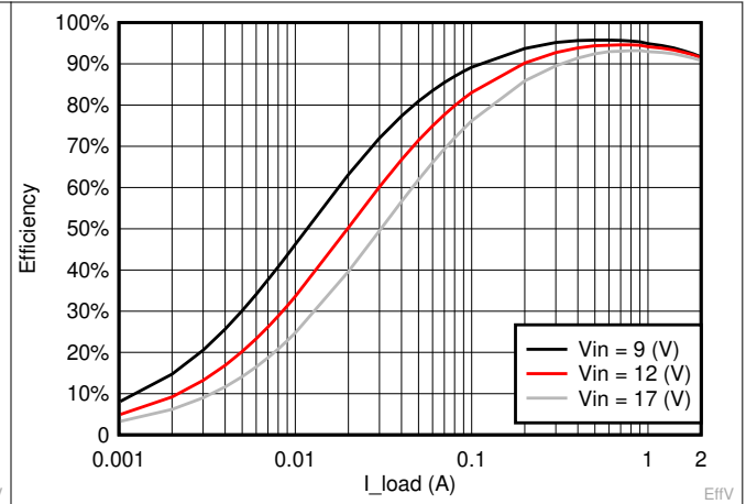
Figure 7-14. V_{OUT} = 5 V Efficiency, L = 4.7 μH
