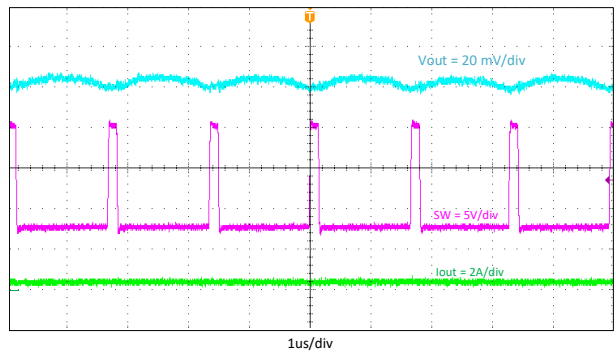
Figure 9-5. Output Voltage Ripple, I_{out} = 0.2\text{ A}
