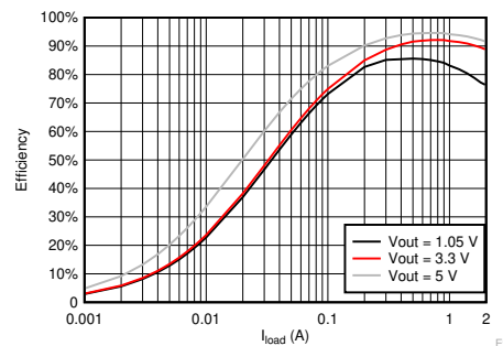
TPS562207S Efficiency
