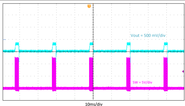
Figure 9-7. Hiccup, I_{out} = 5\text{ A}
