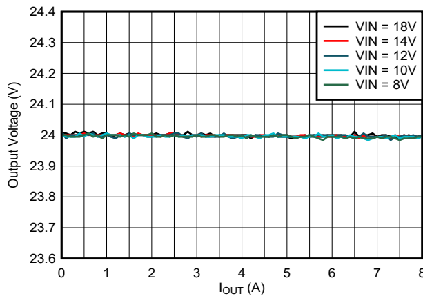
Figure 9-6. 24 V Load Regulation
