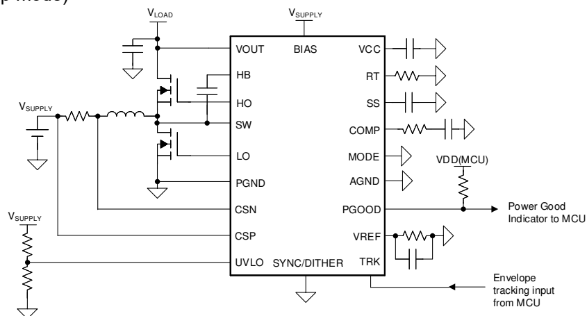
Typical Application
