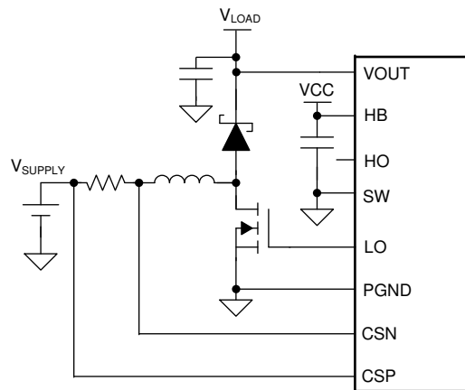
Figure 9-8. Non-synchronous Boost Configuration
