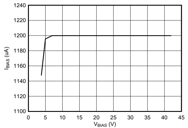
Figure 7-4. V BIAS vs I BIAS (Active Mode)
