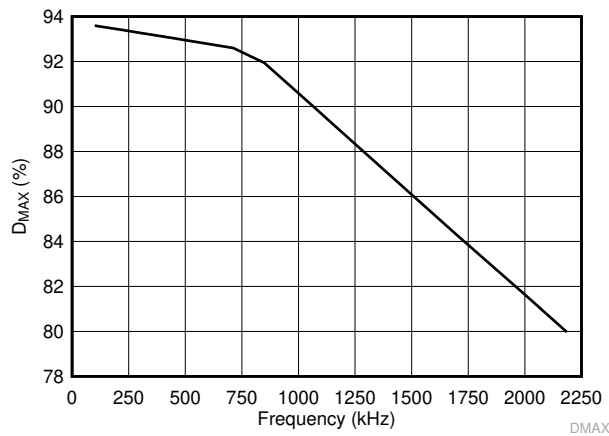
Figure 7-17. D_{MAX} vs Frequency
