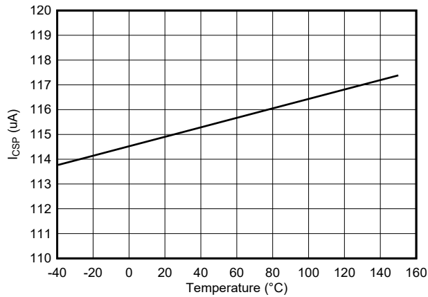
Figure 7-13. I_{CSP} vs Temperature (Active Mode)
