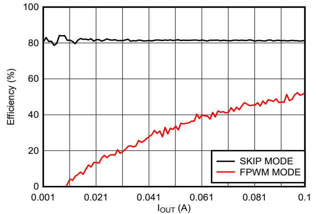
Figure 9-5. Efficiency vs. I_{OUT} , V_{OUT} = 24\text{ V} Light Load
