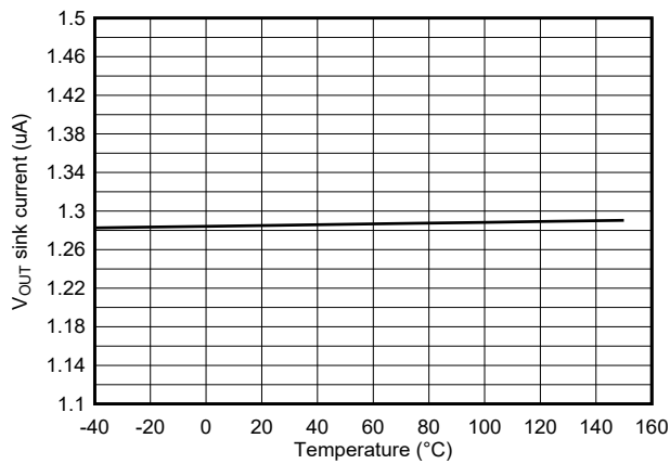
Figure 7-15. V_{OUT} Sink Current vs Temperature (Deep Sleep)
