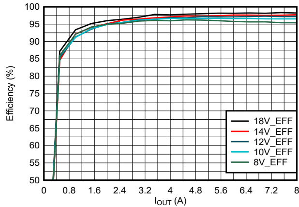
Figure 9-4. Efficiency vs. I_{OUT} , V_{OUT} = 24\text{ V} (FPWM)
