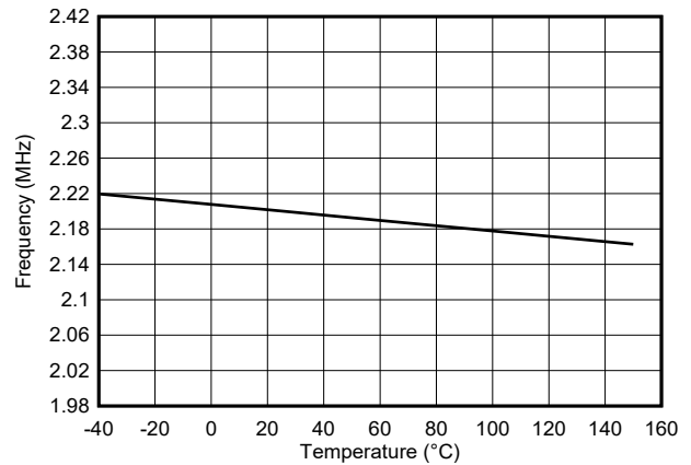
Figure 7-2. Frequency vs Temperature (RT = 9.09 kΩ, 2.2 MHz)
