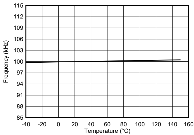
Figure 7-3. Frequency vs Temperature (RT = 220 kΩ, 100 kHz)
