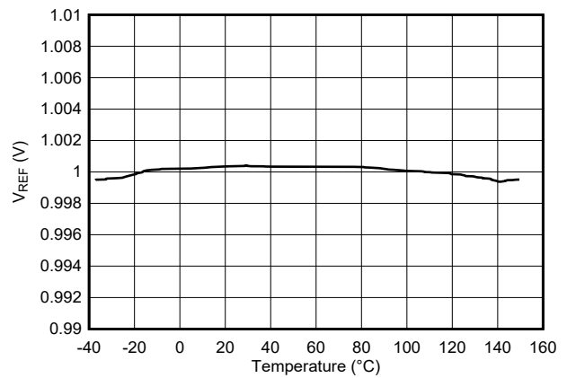
Figure 7-16. V_{REF} vs Temperature
