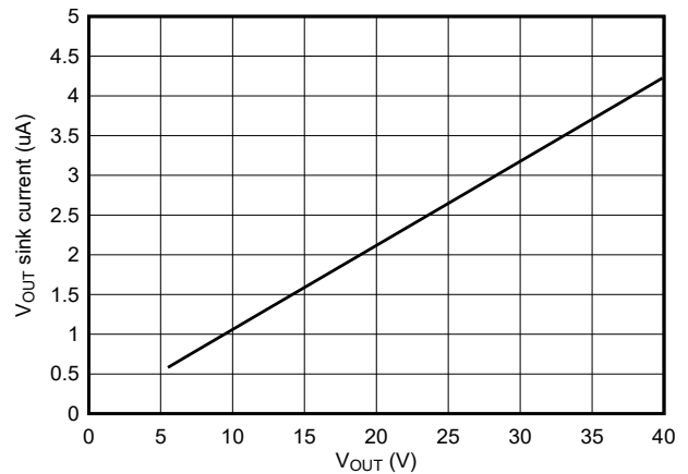
Figure 7-14. V_{OUT} Sink Current vs V_{OUT} (Deep Sleep)
