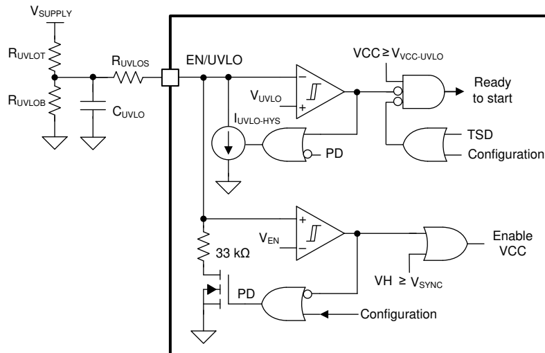
Figure 8-1. EN/UVLO Circuit
