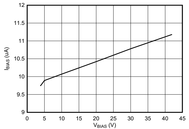
Figure 7-6. V BIAS vs I BIAS (Bypass Mode, Charge Pump Off)
