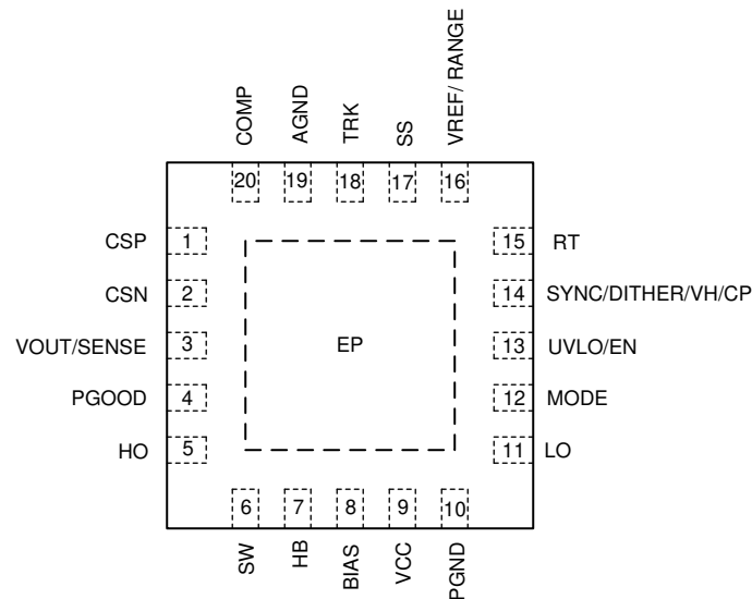
20-Pin QFN with Wettable Flanks RGR Package (Top View)
