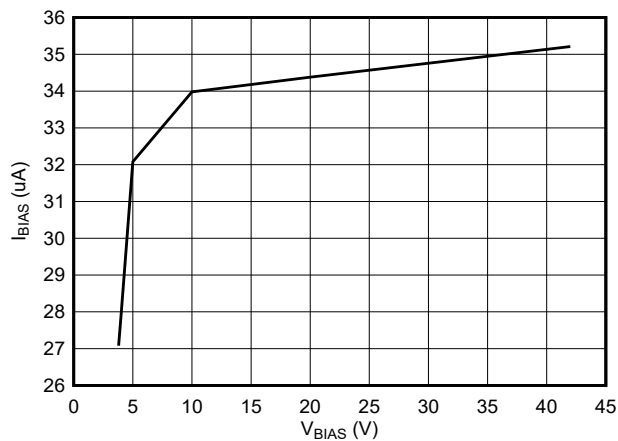
Figure 7-5. V BIAS vs I BIAS (Bypass Mode, Charge Pump On)
