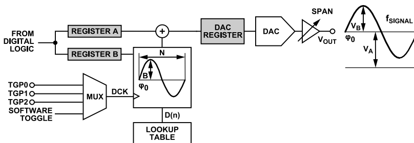
Figure 55. Dither Signal Operation
