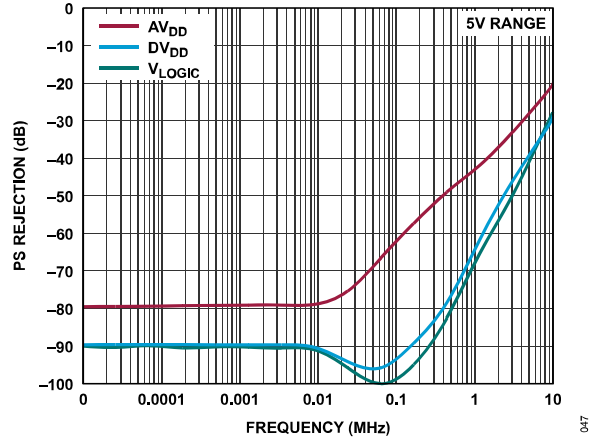
Figure 58. AC PSRR
