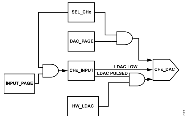
Figure 88. DAC Data Flow Between Registers
