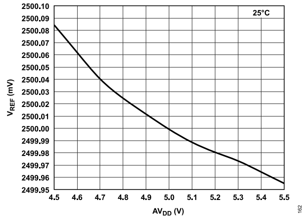
Figure 60. V_{REF} vs. Supply ( AV_{DD} )
