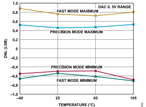
Figure 24. DNL vs. Temperature
