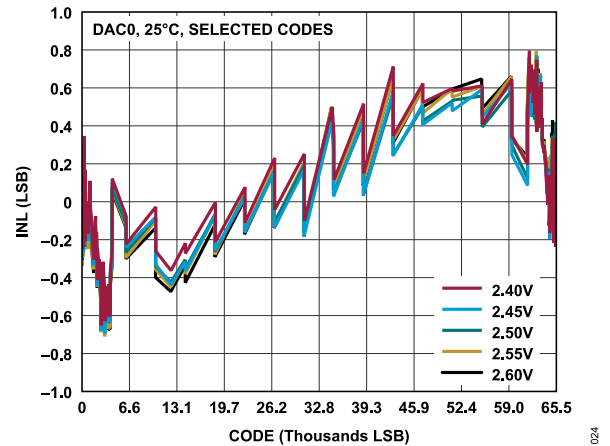
Figure 23. INL vs. Code, Reference Voltage
