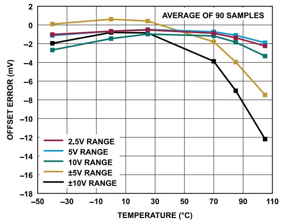
Figure 29. Offset Error vs. Temperature
