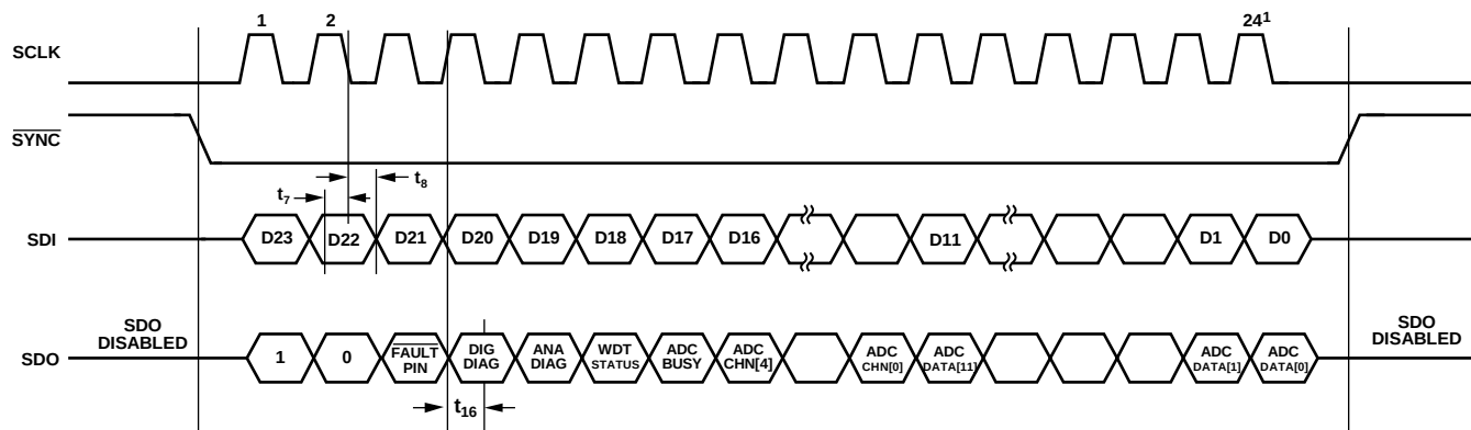
Figure 4. Autostatus Readback
