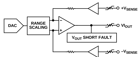
Figure 75. Voltage Output
