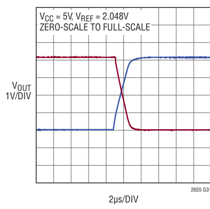
Large-Signal Response
