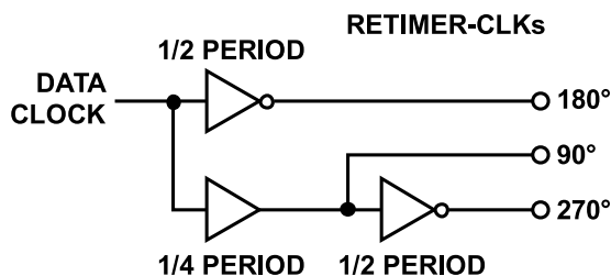
Figure 95. RETIMER-CLK Phases
