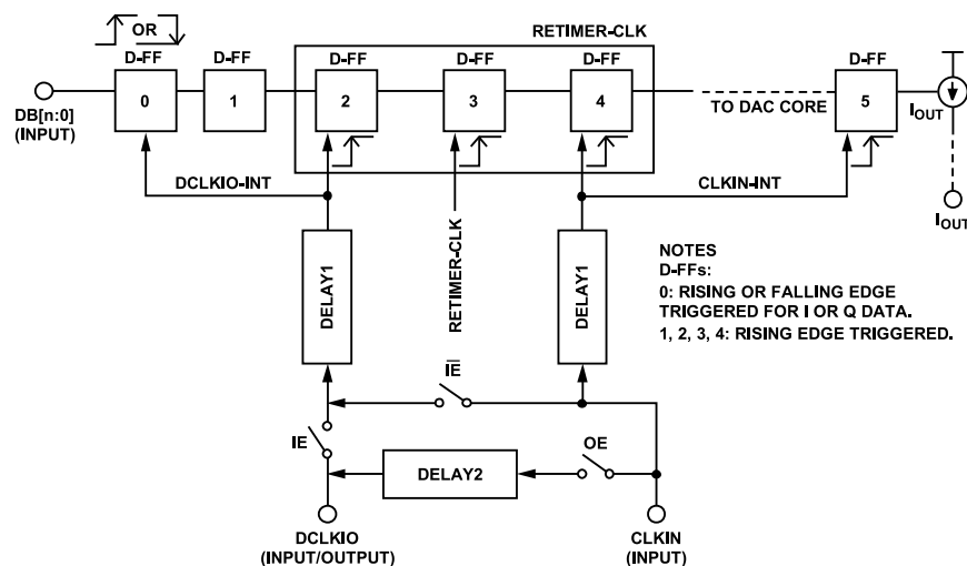
Figure 94. Simplified Diagram of AD9114/AD9115/AD9116/AD9117 Timing
