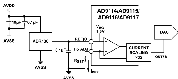
Figure 97. External Reference Configuration
