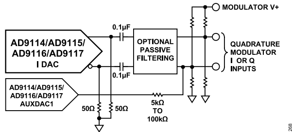
Figure 108. Typical Use of Auxiliary DACs
