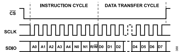
Figure 88. Serial Register Interface Timing, LSB First Read
