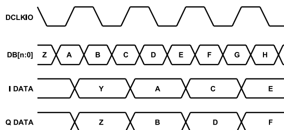
Figure 92. Timing Diagram with IFIRST = 1, IRISING = 1
