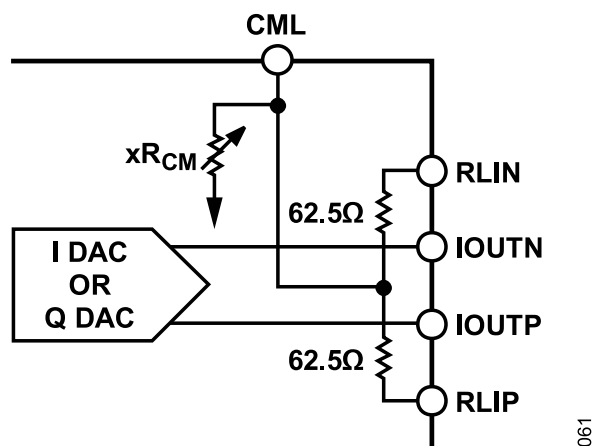
Figure 101. Simplified Internal Load Options
