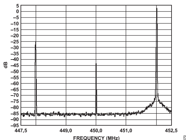
Figure 110. AD9114/AD9115/AD9116/AD9117 and ADL5370 with a Single-Tone Signal at 450 MHz, No Gain or LO Compensation
