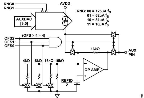
Figure 106. AUXDAC Simplified Circuit Diagram
