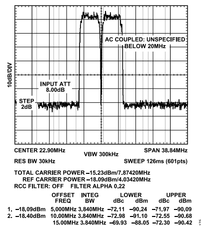
Figure 75. AD9117 ACLR Two-Carrier, 3.3 V
