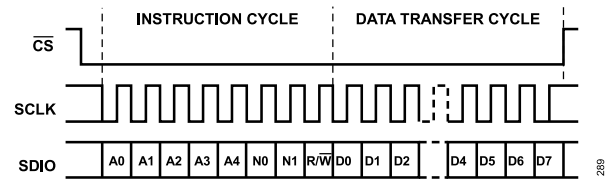
Figure 87. Serial Register Interface Timing, LSB First Write
