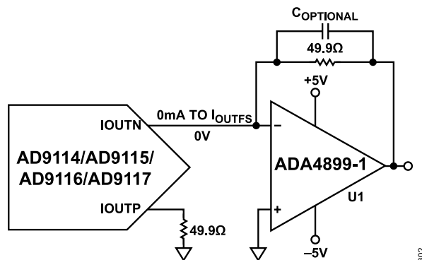
Figure 104. Unipolar Buffered Voltage Output
