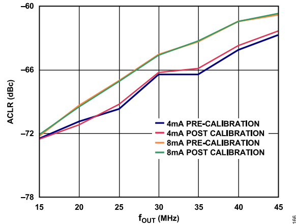
Figure 66. AD9117 One-Carrier W-CDMA First ACLR vs. f_{OUT} , 1.8 V
