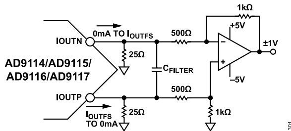
Figure 105. Differential Buffered Voltage Output
