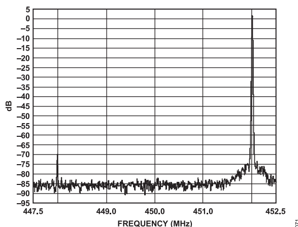
Figure 111. AD9114/AD9115/AD9116/AD9117 and ADL5370 with a Single-Tone Signal at 450 MHz, Gain and LO Compensation Optimized
