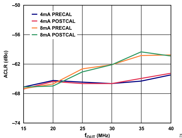
Figure 74. AD9117 Two-Carrier W-CDMA Second ACLR vs. f_{OUT} , 1.8 V
