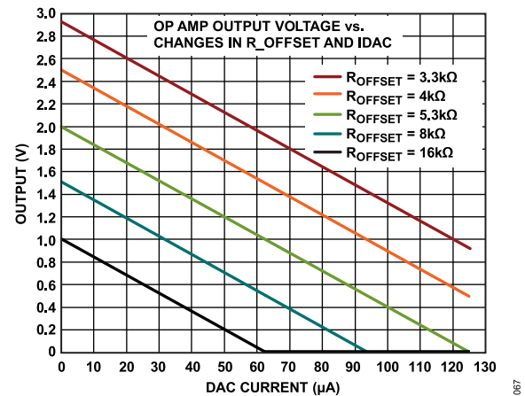
Figure 107. AUXDAC Op Amp Output vs. Current, AVDD = 3.3 V No Load, AUXDAC 0x1FF to 0x000
