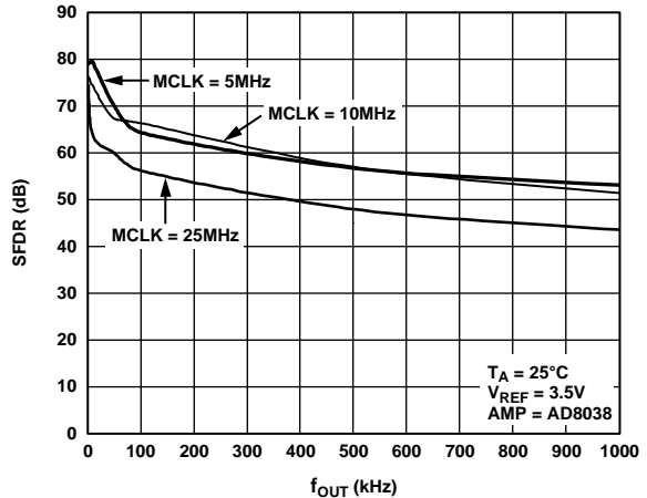
Figure 22. Wideband SFDR vs. f_{OUT} Frequency
