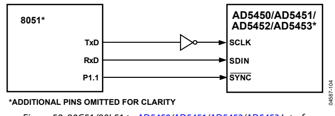
Figure 59. 80C51/80L51 to AD5450/AD5451/AD5452/AD5453 Interface
