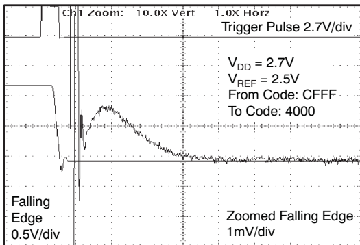
Time (2µs/div) 2.7 V
