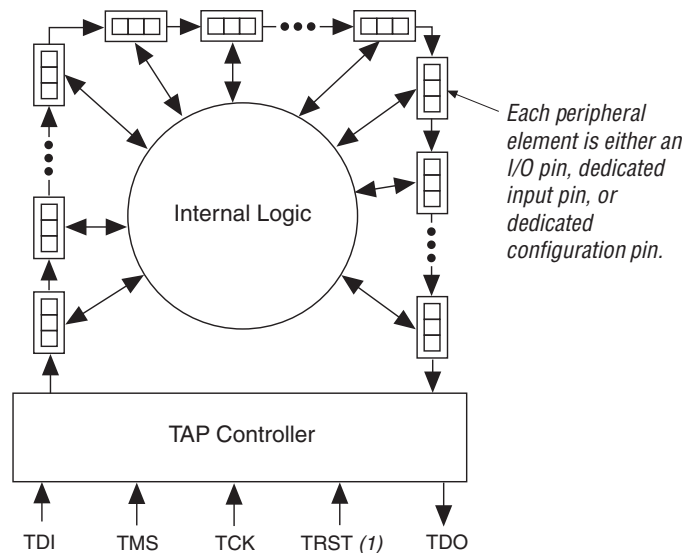
Figure 9–3. Boundary-Scan Register
