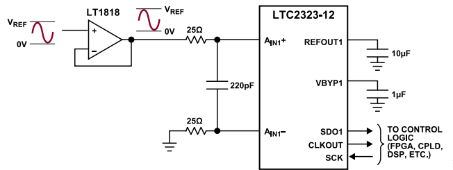
Figure 28. Pseudo-Differential Unipolar Application Circuit
