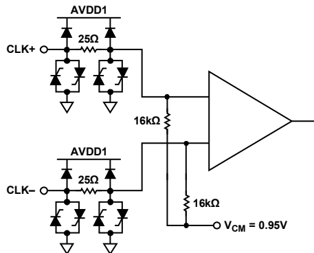
Figure 33. Clock Inputs
