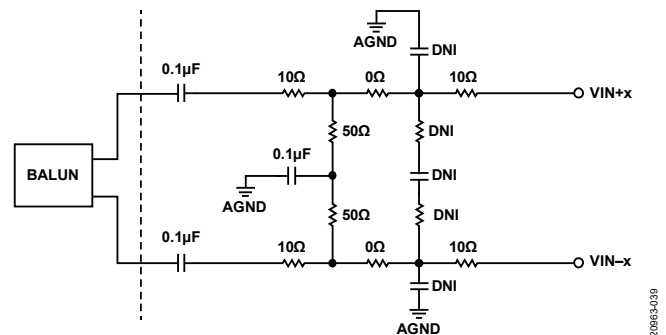
Figure 44. Differential Transformer Coupled Configuration for A_{IN} > 735\text{ MHz}
