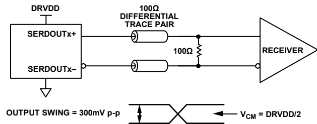
Figure 65. DC-Coupled Digital Output Termination Example
