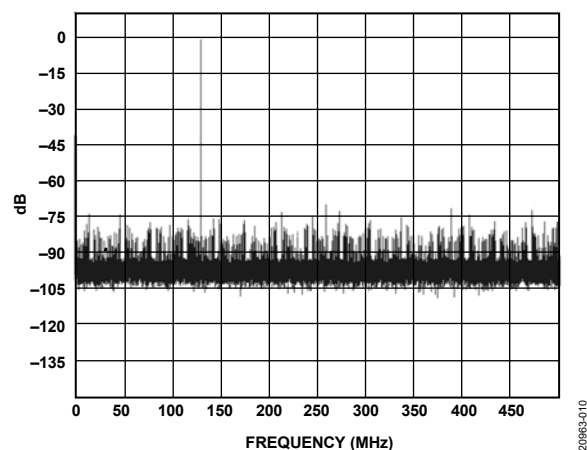
Figure 10. Single-Tone FFT with f_{IN} = 871 MHz, SNRFS = 48.5 dBFS, SFDR = 70 dBFS, SINAD = 48.5 dBFS
