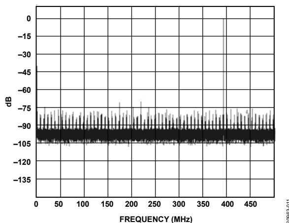
Figure 11. Single-Tone FFT with f_{IN} = 1391 MHz, SNRFS = 48.4 dBFS, SFDR = 70 dBFS, SINAD = 48.4 dBFS
