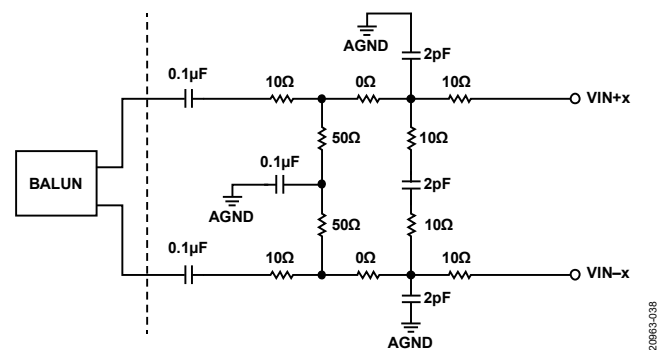
Figure 43. Differential Transformer Coupled Configuration A_{IN} \leq 735\text{ MHz}
