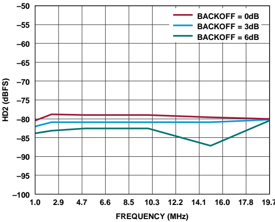
Figure 20. ADC HD2 vs. Frequency at Various Backoff Values and A_{IN} = -2 dB, 1 GSPS
