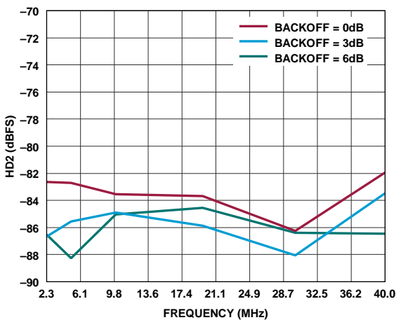
Figure 21. ADC HD2 vs. Frequency at Various Backoff Values and A_{IN} = -2 dB, 2 GSPS
