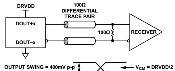
Figure 67. DC-Coupled Digital Output Termination Example
