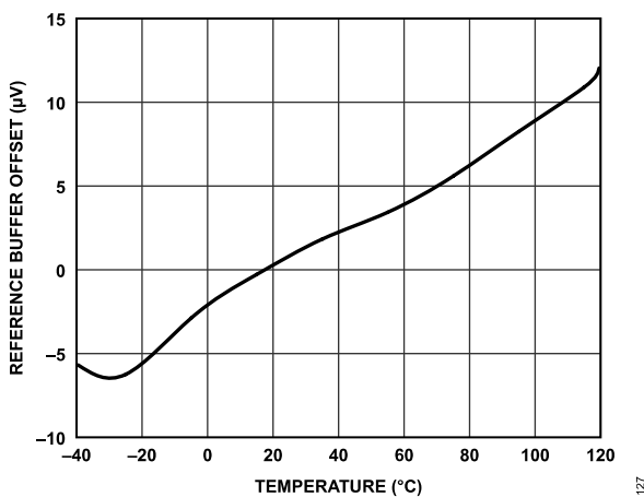
Figure 26. Reference Buffer Offset vs. Temperature
