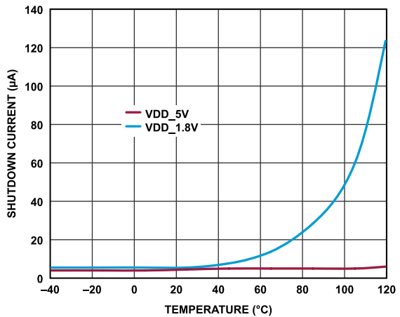
Figure 35. Shutdown Current vs. Temperature
