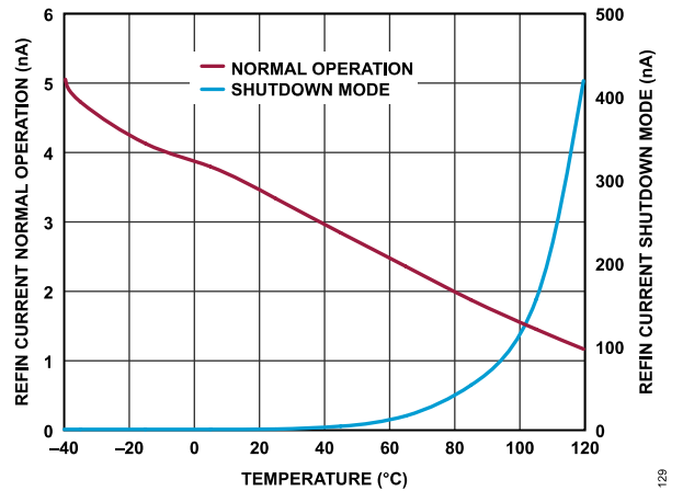
Figure 28. REFIN Current Normal Operation and REFIN Current Shutdown Mode vs. Temperature
