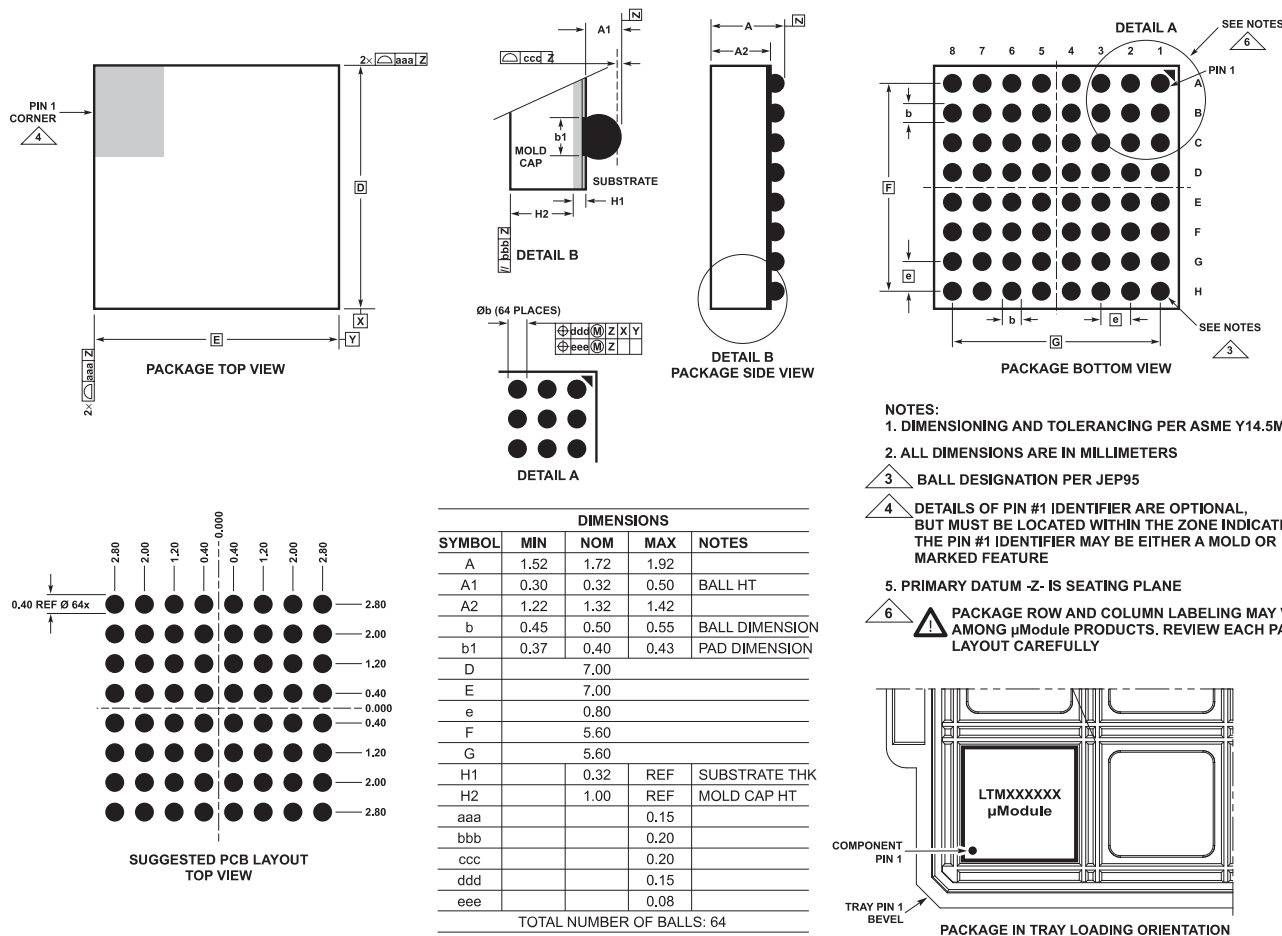
Figure 57. 64-Ball Chip Scale Package Ball Grid Array [CSP_BGA] (BC-64-8) Dimensions shown in millimeters
