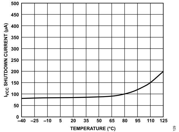
Figure 28. I_{VCC} Shutdown Current vs. Temperature
