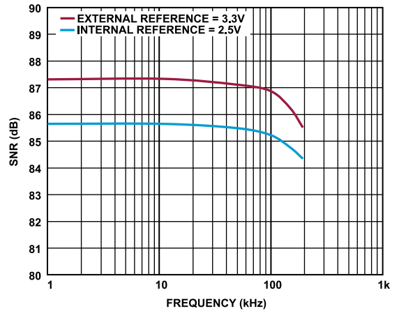
Figure 18. AD4683 SNR vs. Frequency
