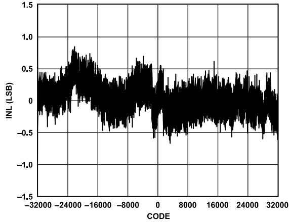
Figure 13. Typical INL Error
