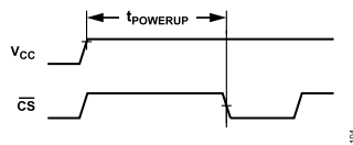
Figure 4. Power-Up Time to Conversion
