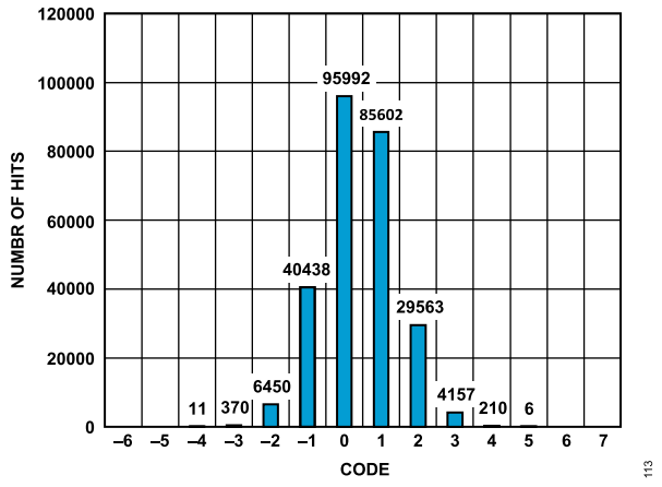
Figure 12. DC Histogram at Code Center
