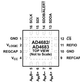
Figure 6. Pin Configuration
