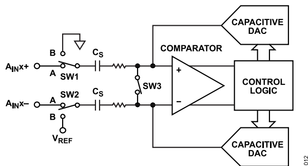
Figure 31. ADC Acquisition Phase
