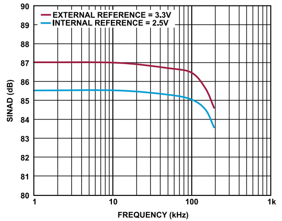
Figure 17. AD4682 SINAD vs. Frequency
