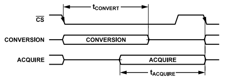
Figure 3. Internal Conversion Acquire Timing
