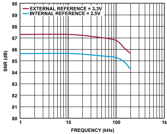
Figure 14. AD4682 SNR vs. Frequency
