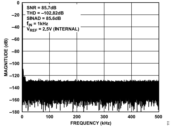
Figure 10. AD4682 FFT, V_{REF} = 2.5\text{ V Internal}
