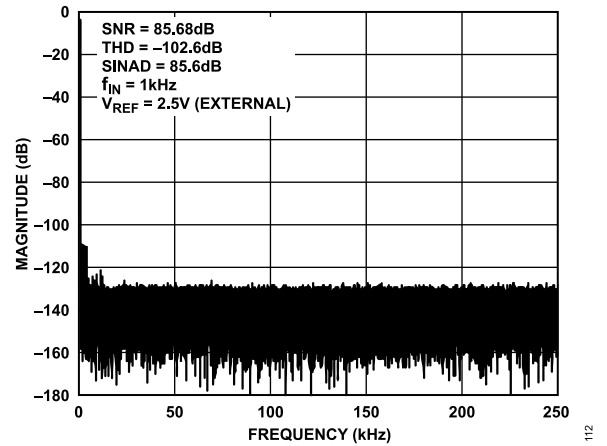
Figure 11. AD4683 FFT, V_{REF} = 2.5\text{ V External}
