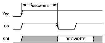
Figure 5. Power-Up Time to Register Read Write Access
