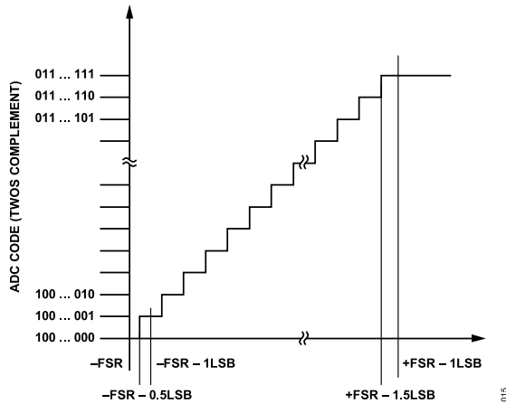
Figure 31. ADC Ideal Transfer Function (FSR = Full-Scale Range)
