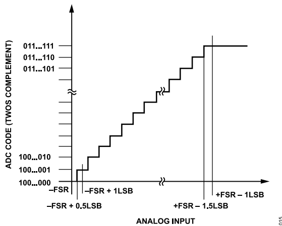
Figure 34. ADC Ideal Transfer Function (FSR = Full-Scale Range)
