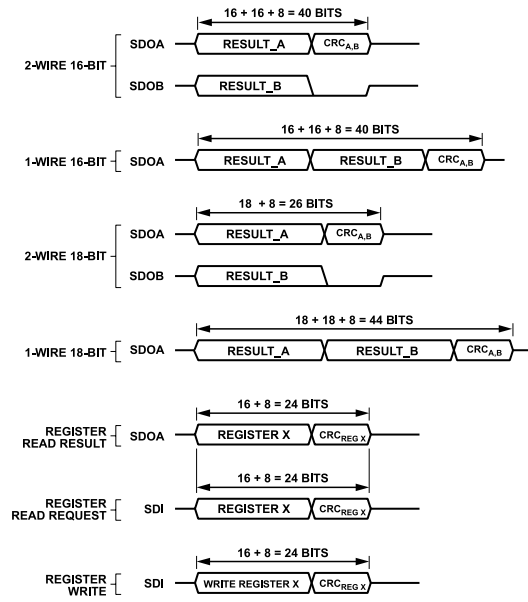
Figure 46. CRC Operation
