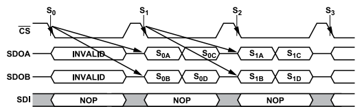
Figure 38. Read Conversion Results, 2-Wire Mode
