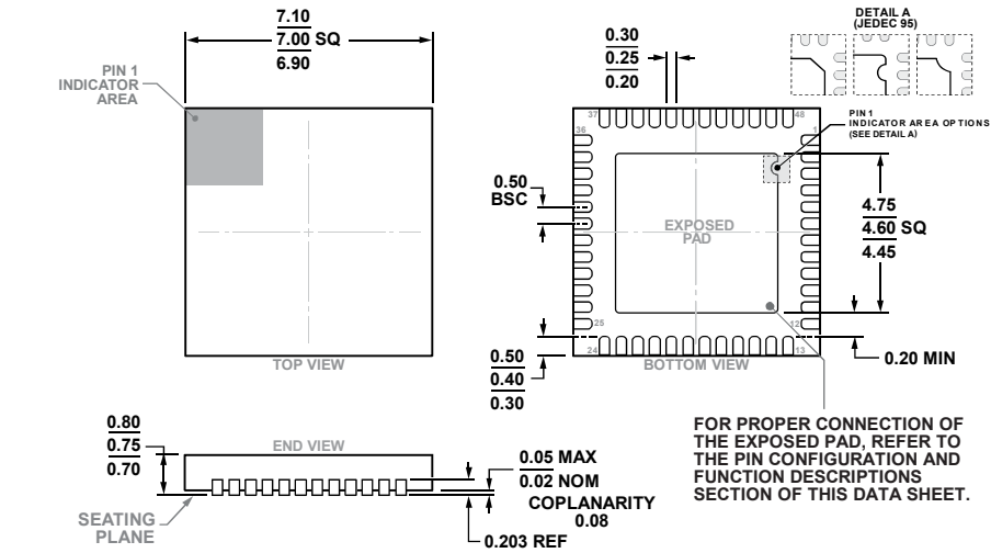
COMPLIANT TO JEDEC STANDARDS MO-220-WKGD-2 Figure 26. 48-Lead Lead Frame Chip Scale Package [LFCSP] 7 mm × 7 mm Body and 0.75 mm Package Height (CP-48-14) Dimensions shown in millimeters
